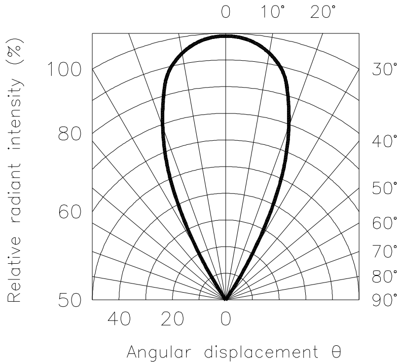
Radiation Diagram
