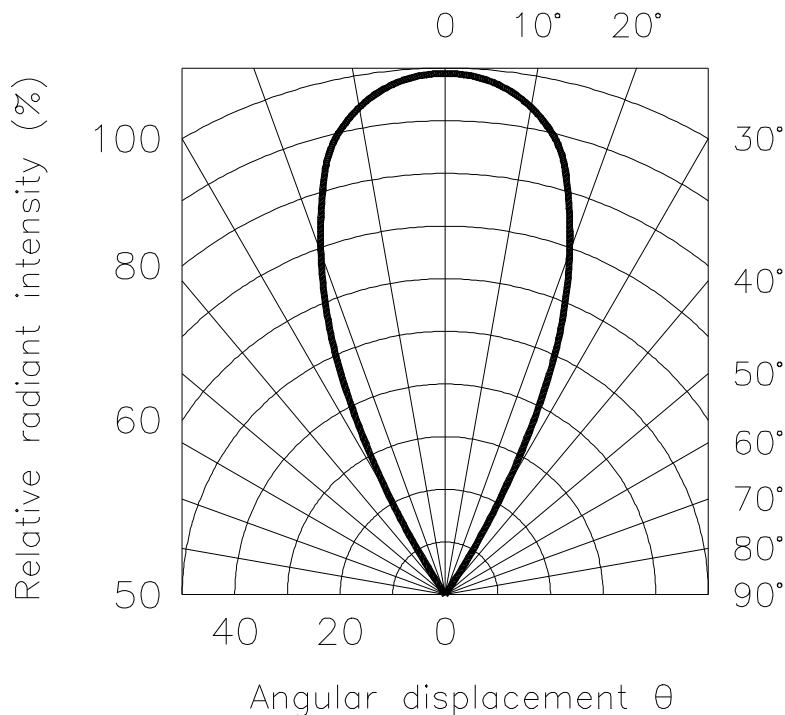
Radiation Diagram
