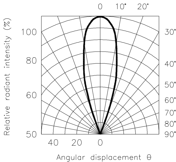
Radiation Diagram
