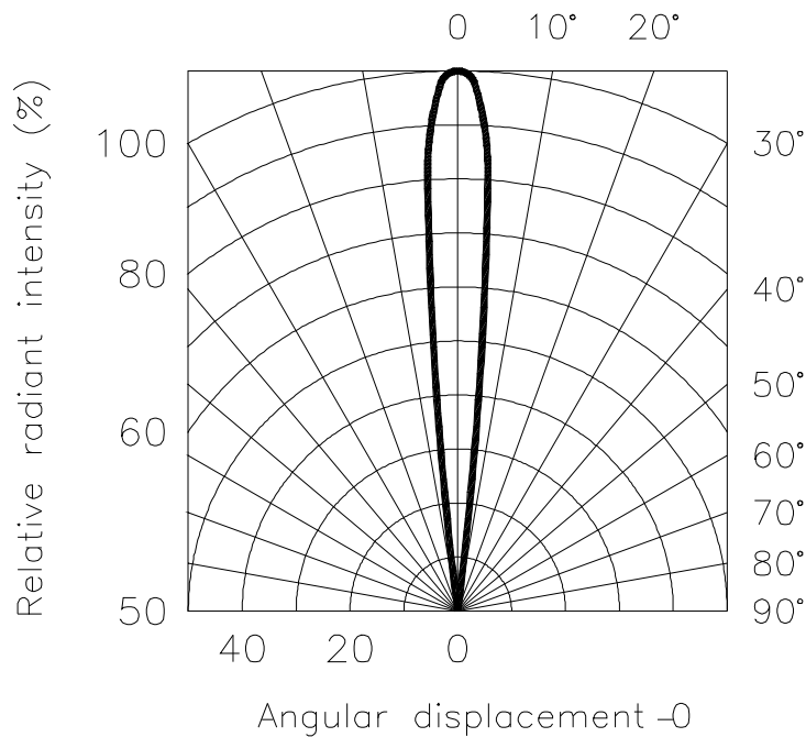
Radiation Diagram
