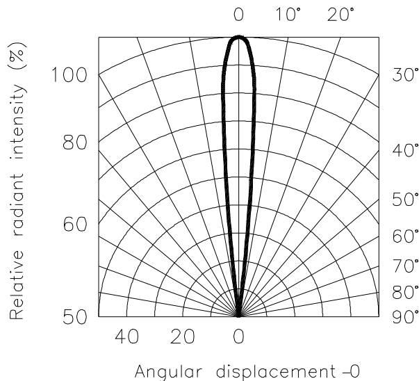
Radiation Diagram
