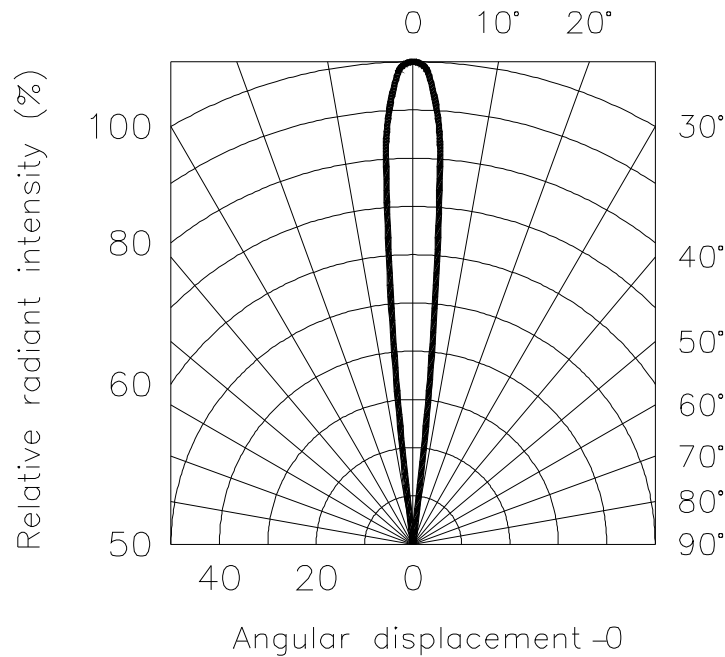
Radiation Diagram
