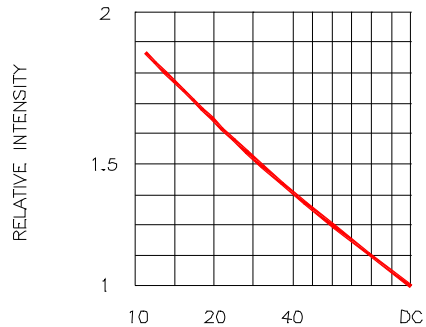
Fig.4 LUMINOUS INTENSITY VS. DUTY CYCLE
