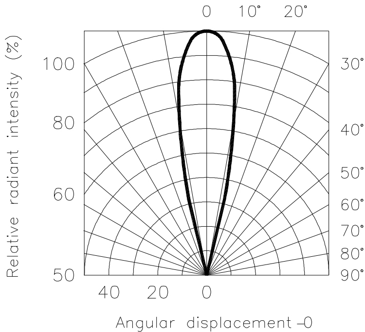
Radiation Diagram
