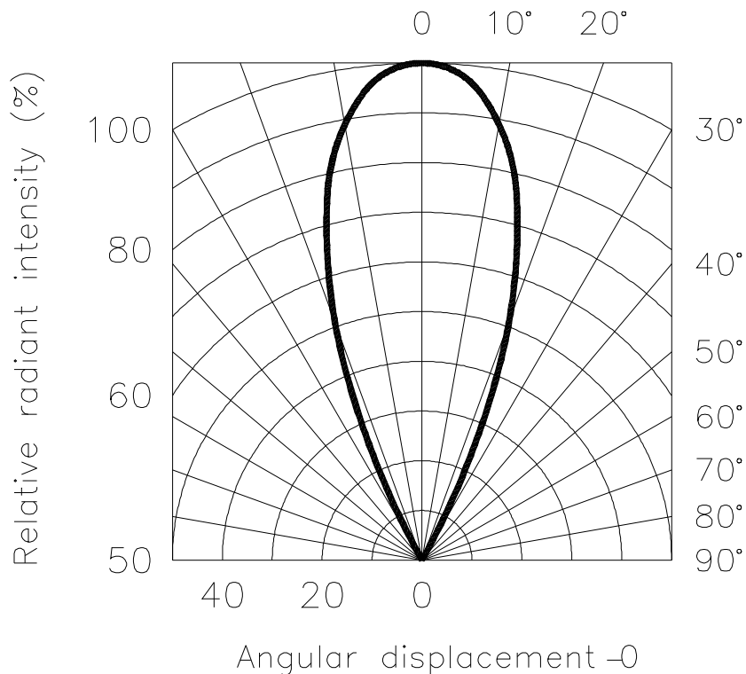
Radiation Diagram
