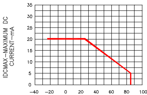
Fig.5 MAXIMUM ALLOWABLE DC CURRENT PER SEGMENT VS. AMBIENT TEMPERATURE
